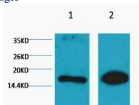
Western blot analysis of 1) Rat Testis Tissue, 2) Raw264.7 diluted at 1:1000.
